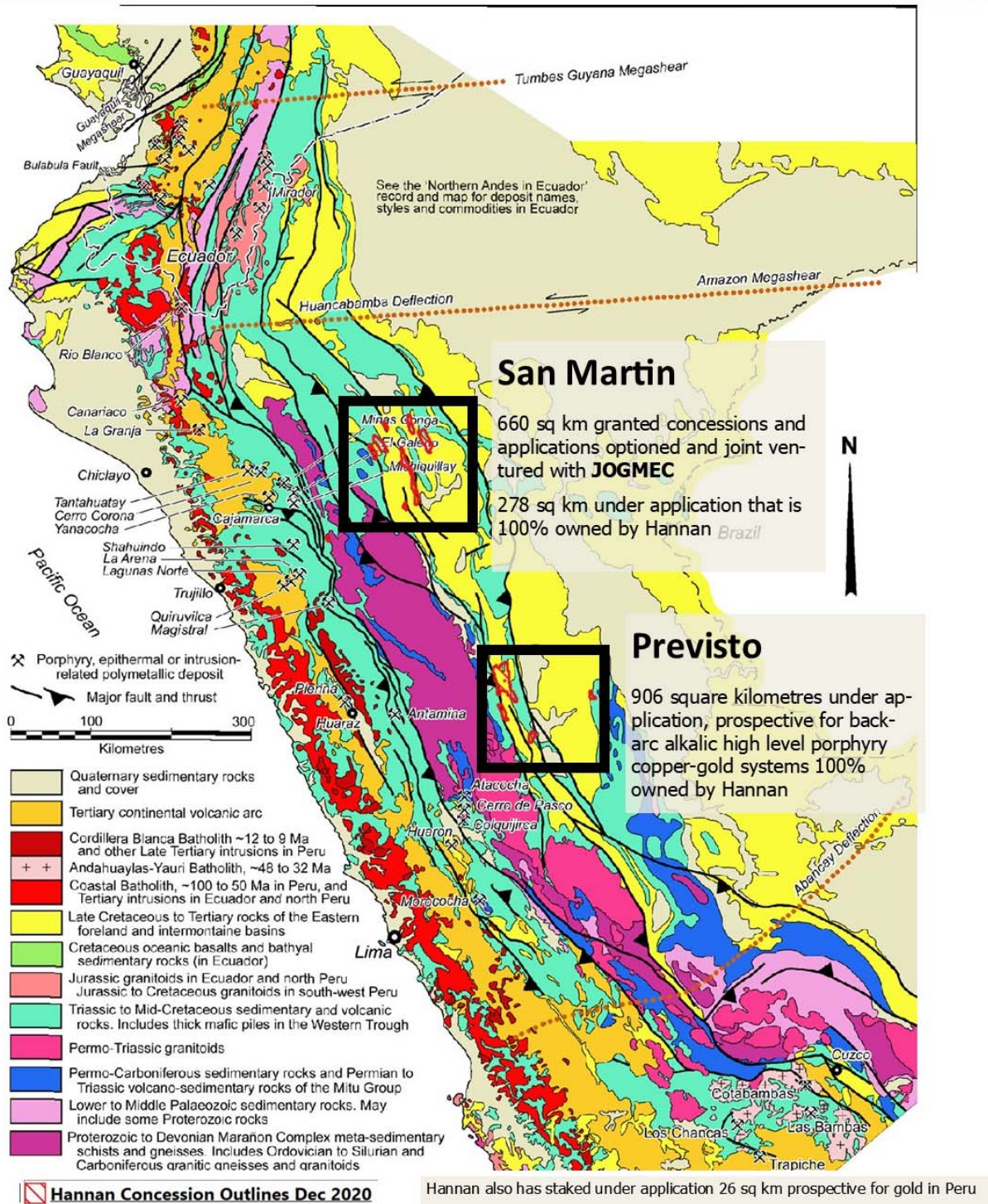
Figure 1. Hannan Metals mineral concessions in context with the tectonic and geological setting of porphyry Cu-Au-Mo, epithermal Au/Ag and intrusion-related polymetallic Zn-Pb-Cu-Ag deposits in the Peruvian Andes.
