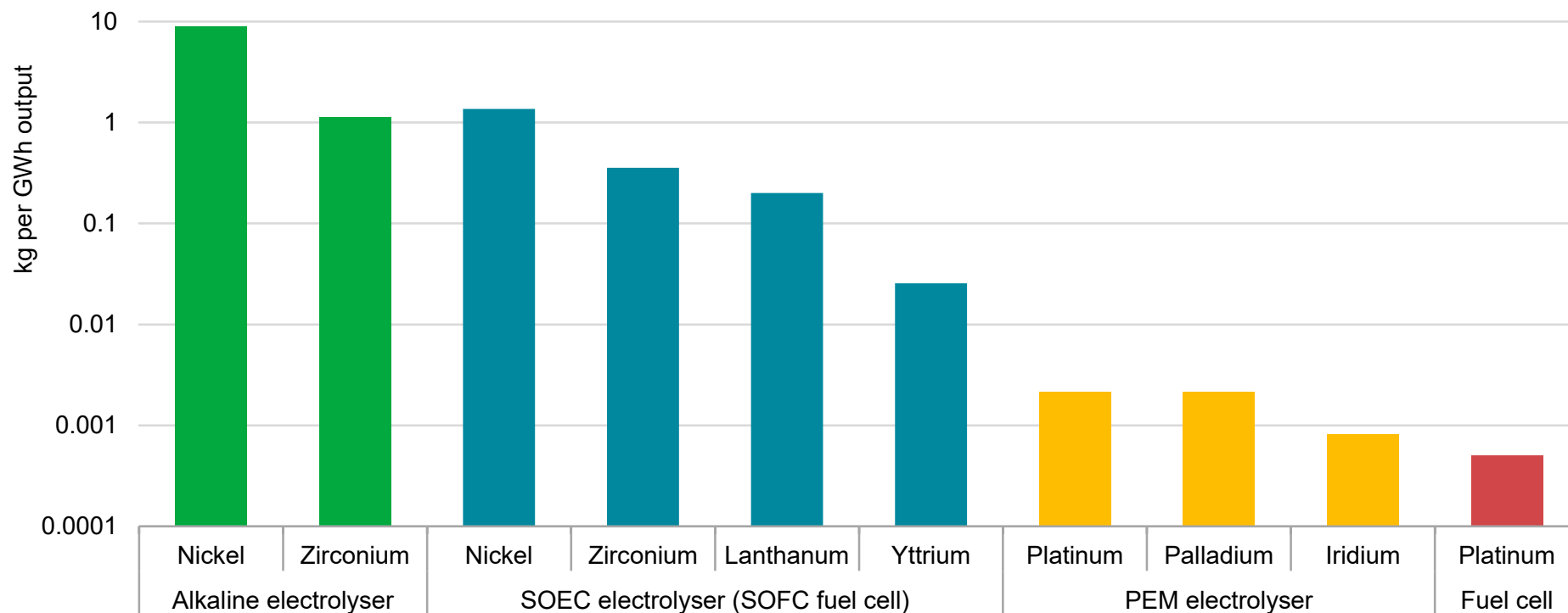
Estimated levelised demand for selected minerals in electrolyzers and fuel cells today
